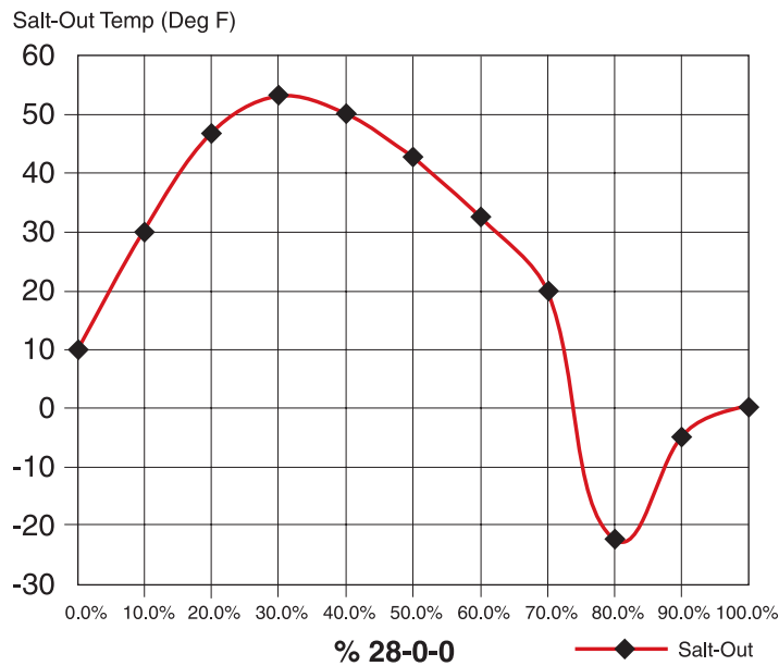
Salt-Out Temperature (Deg F.) vs % 28-0-0 in GoldStart 6-24-6
